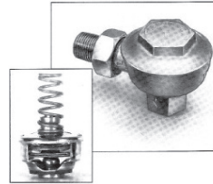
THERMOSTATIC STEAM TRAPS For Low & Moderate Pressure Service
