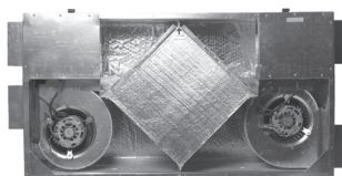
NU0508 Light Commercial HRV
