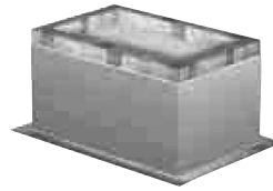
GPI ROOF CURBS FOR FLAT ROOFS c/w Galvanized Construction, 1" Insulation, 2" Flashing Flange & 12" High
